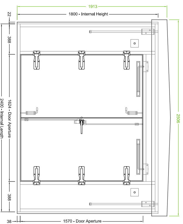
FRONT ELEVATION
