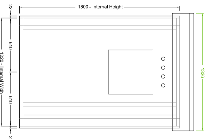
RH SIDE ELEVATION
